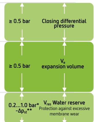
Reflex vessels
