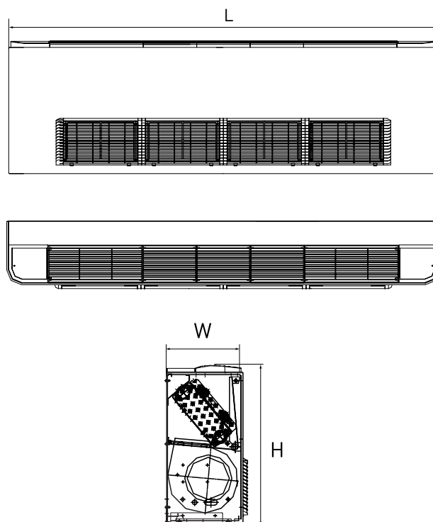
WITH CASING
