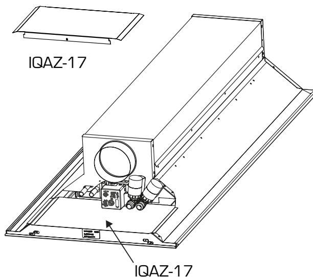
Figure 9: IQAZ-17 cross talk protection plate
