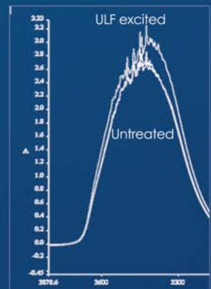
Water internal energy excitation by ULF
