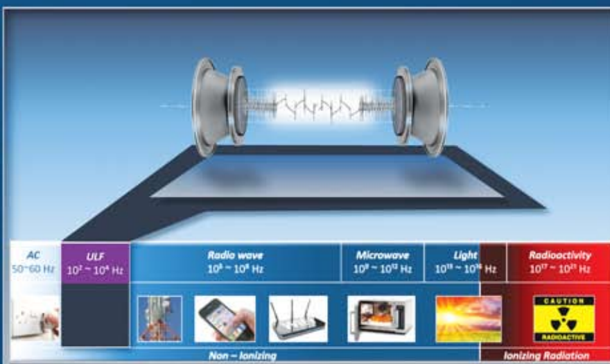
ULF frequency range in electromagnetic wave spectrum
