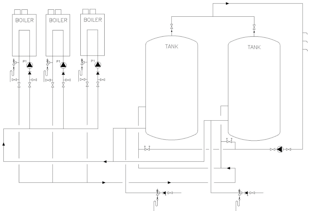
Three water heaters with two storage tanks
